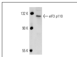
eIF3 p110 (A-20): sc-31872. Western blot analysis of eIF3 p110 expression in F9 whole cell lysate.
