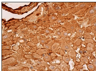
Ras GAP (P-16): sc-32049. Immunoperoxidase staining of formalin fixed, paraffin-embedded human placenta tissue showing cytoplasmic and membrane staining of decidual cells.
