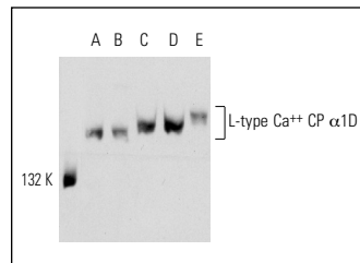
L-type Ca ++ CP α1D (E-19): sc-32072. Western blot analysis of L-type Ca ++ CP α1D expression in L6 (A), C6 (B), IMR-32 (C), SK-N-SH (D) and U-87 MG (E) whole cell lysates.
