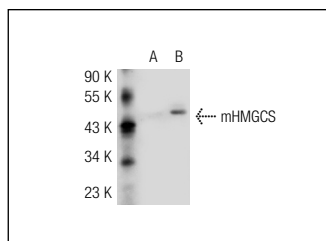
mHMGCS (D-17): sc-32425. Western blot analysis of mHMGCS expression in non-transfected: sc-117752 (A) and mouse mHMGCS transfected: sc-121641 (B) 293T whole cell lysates.
