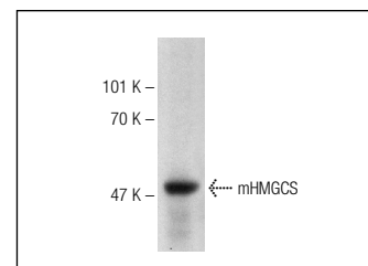
mHMGCS (D-17): sc-32425. Western blot analysis of mHMGCS expression in mouse liver tissue extract.
