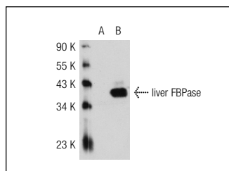
liver FBPase (N-13): sc-32430. Western blot analysis of liver FBPase expression in non-transfected: sc-117752 (A) and human liver FBPase transfected: sc-113796 (B) 293T whole cell lysates.
