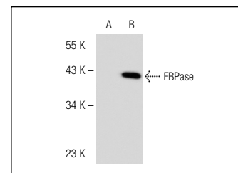
liver FBPase (N-13): sc-32430. Western blot analysis of FBPase expression in non-transfected: sc-117752 (A) and human FBPase transfected: sc-113796 (B) 293T whole cell lysates.
