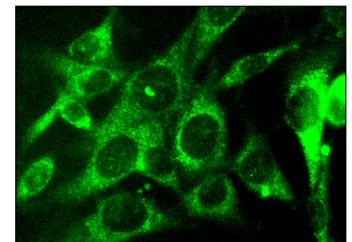
muscle FBPase (C-12): sc-32438. Immunofluorescence staining of methanol-fixed Sol8 cells showing cytoplasmic localization.
