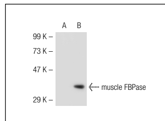
muscle FBPase (C-12): sc-32438. Western blot analysis of muscle FBPase expression in non-transfected: sc-117752 (A) and mouse muscle FBPase transfected: sc-121871 (B) 293T whole cell lysates.
