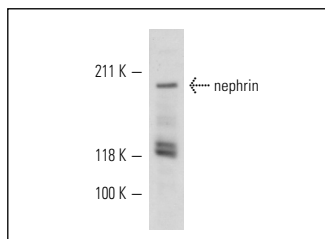
nephrin (N-16): sc-32532. Western blot analysis of nephrin expression in KNRK whole cell lysate.
