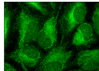
nephrin (N-16): sc-32532. Immunofluorescence staining of formalin-fixed HeLa cells showing cytoplasmic localization.
