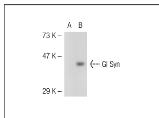
GI Syn (G-20): sc-32560. Western blot analysis of GI Syn expression in non-transfected: sc-117752 (A) and mouse GI Syn transfected: sc-120492 (B) 293T whole cell lysates.
