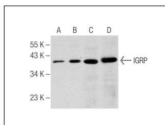
IGRP (C-19): sc-33473. Western blot analysis of IGRP expression in non-transfected: sc-117752 (A) and human IGRP transfected: sc-373081 (B) 293T whole cell lysates and mouse pancreas (C) and mouse thymus (D) tissue extracts.
