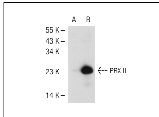
PRX II (M-40): sc-33572. Western blot analysis of PRX II expression in non-transfected: sc-117752 (A) and mouse PRX II transfected: sc-122808 (B) 293T whole cell lysates.
