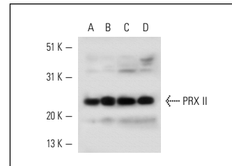
PRX II (M-40): sc-33572. Western blot analysis of PRX II expression in SK-BR-3 (A), SK-N-SH (B), MDA-MB-231 (C) and MCF7 (D) whole cell lysates.
