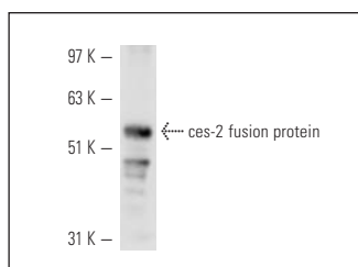
ces-2 (ce-211): sc-33739. Western blot analysis of C. elegans recombinant ces-2 fusion protein.
