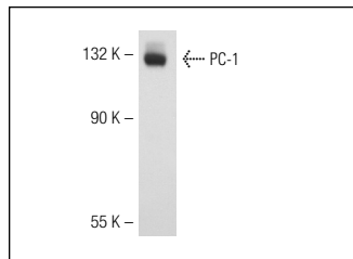
PC-1 (H-120): sc-33813. Western blot analysis of PC-1 expression in Hep G2 whole cell lysate.
