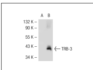
TRB-3 (T-15): sc-34213. Western blot analysis of TRB-3 expression in non-transfected: sc-117752 (A) and mouse TRB-3 transfected: sc-127703 (B) 293T whole cell lysates.
