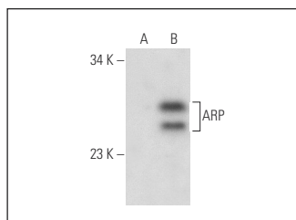
ARP (P-13): sc-34563. Western blot analysis of ARP expression in non-transfected: sc-117752 (A) and human ARP transfected: sc-373148 (B) 293T whole cell lysates.
