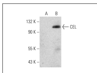
CEL (D-20): sc-34878. Western blot analysis of CEL expression in non-transfected: sc-117752 (A) and human CEL transfected: sc-115618 (B) 293T whole cell lysates.
