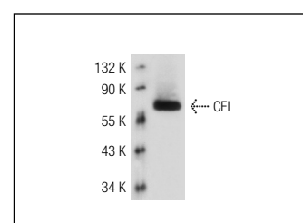
CEL (D-20): sc-34878. Western blot analysis of CEL expression in mouse pancreas tissue extract.
