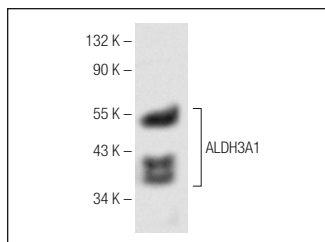
ALDH3A1 (A-5): sc-373688. Western blot analysis of ALDH3A1 expression in A549 whole cell lysate.
