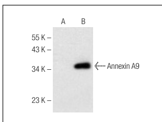
Annexin A9 (B-11): sc-373933. Western blot analysis of Annexin A9 expression in non-transfected: sc-117752 (A) and mouse Annexin A9 transfected: sc-118427 (B) 293T whole cell lysates.
