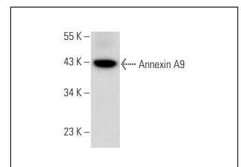
Annexin A9 (B-11): sc-373933. Western blot analysis of Annexin A9 expression in rat kidney tissue extract.
