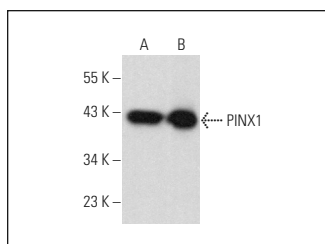
PINX1 (E-9): sc-374115. Western blot analysis of PINX1 expression in A549 whole cell lysate (A) and K-562 nuclear extract (B).
