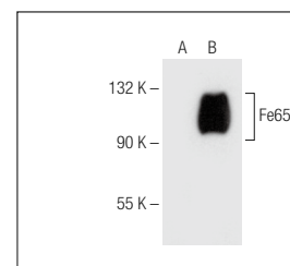
Fe65 (D-11): sc-374641. Western blot analysis of Fe65 expression in non-transfected: sc-117752 (A) and human Fe65 transfected: sc-175237 (B) 293T whole cell lysates.
