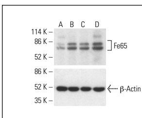
Fe65 (D-11): sc-374641. Western blot analysis of Fe65 expression in untreated (A) and chemically-treated (B, C, D) HEK293T whole cell lysates. Detection reagent used: m-IgG \kappa BP-HRP: sc-516102. \beta -Actin (C4): sc-47778 used as loading control. Detection reagent used: m-IgG Fc BP-HRP: sc-525409.
