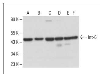
Int-6 (H-5): sc-376110. Western blot analysis of Int-6 expression in KNRK (A), RPE-J (B), Daudi (C), K-562 (D), NIH/3T3 (E) and C3H/10T1/2 (F) whole cell lysates.
