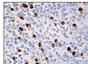
Ndfip2 (E-4): sc-376259. Immunoperoxidase staining of formalin fixed, paraffin-embedded human tonsil tissue showing cytoplasmic staining of subset of cells in non-germinal center.
