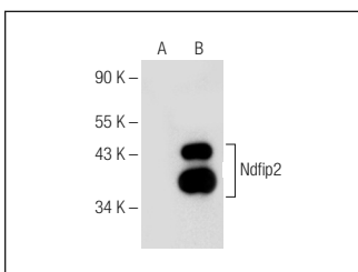
Ndfip2 (E-4): sc-376259. Western blot analysis of Ndfip2 expression in non-transfected: sc-117752 (A) and mouse Ndfip2 transfected: sc-121960 (B) 293T whole cell lysates.
