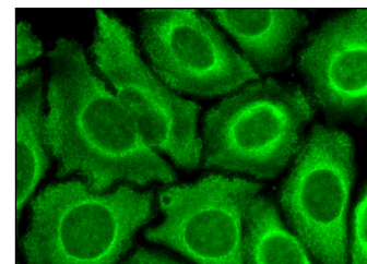
GPI (E-4): sc-398382. Immunofluorescence staining of methanol-fixed HeLa cells showing cytoplasmic and membrane localization.
