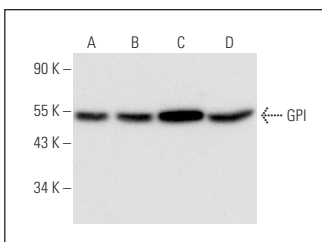
GPI (E-4): sc-398382. Western blot analysis of GPI expression in HEK293 (A), HeLa (B), RT-4 (C) and U-251-MG (D) whole cell lysates.
