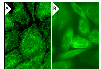
GFR \alpha -3 (C-3): sc-398618. Immunofluorescence staining of formalin-fixed A-431 cells showing membrane localization (A). GFR \alpha -3 (C-3) Alexa Fluor ® 488: sc-398618 AF488. Direct immunofluorescence staining of formalin-fixed SW480 cells showing membrane localization. Blocked with UltraCruz ® Blocking Reagent: sc-516214 (B).
