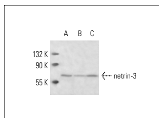
netrin-3 (H-13): sc-46191. Western blot analysis of netrin-3 expression in SK-N-MC (A), U-87 MG (B) and SK-N-SH (C) whole cell lysates.
