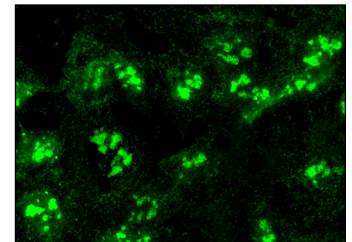
Nucleostemin (P-19): sc-46219. Immunofluorescence staining of formalin-fixed Hep G2 cells showing nucleolar localization.
