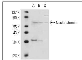
Nucleostemin (P-19): sc-46219. Western blot analysis of Nucleostemin expression in HeLa (A), Hep G2 (B) and LADMAC (C) nuclear extracts.
