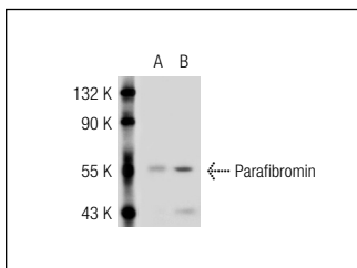
Parafibromin (S-20): sc-46227. Western blot analysis of Parafibromin expression in non-transfected: sc-117752 (A) and human Parafibromin transfected: sc-117050 (B) 293T whole cell lysates.
