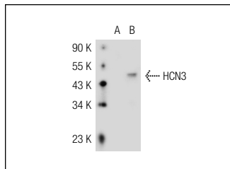
HCN3 (C-13): sc-46353. Western blot analysis of HCN3 expression in non-transfected: sc-117752 (A) and human HCN3 transfected: sc-114783 (B) 293T whole cell lysates.
