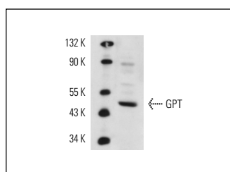
GPT (A-16): sc-47017. Western blot analysis of GPT expression in mouse heart tissue extract.
