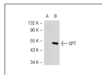
GPT (A-16): sc-47017. Western blot analysis of GPT expression in non-transfected: sc-117752 (A) and mouse GPT transfected: sc-120613 (B) 293T whole cell lysates.
