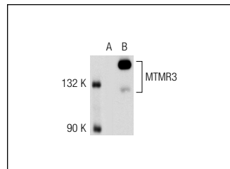
MTMR3 (C-17): sc-47185. Western blot analysis of MTMR3 expression in non-transfected: sc-117752 (A) and human MTMR3 transfected: sc-112826 (B) 293T whole cell lysates.
