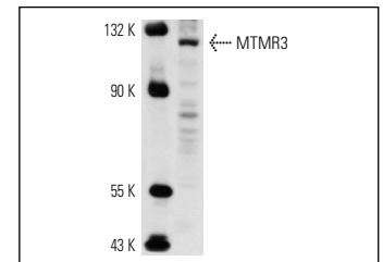
MTMR3 (C-17): sc-47185. Western blot analysis of MTMR3 expression in Sol 8 nuclear extract.
