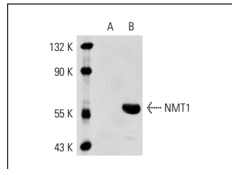
NMT1 (P-18): sc-47213. Western blot analysis of NMT1 expression in non-transfected: sc-110760 (A) and human NMT1 transfected: sc-110896 (B) 293 whole cell lysates
