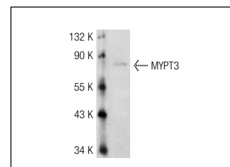
MYPT3 (K-14): sc-47343. Western blot analysis of MYPT3 expression in mouse brain tissue extract.
