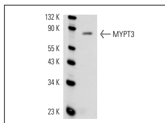
MYPT3 (K-14): sc-47343. Western blot analysis of MYPT3 expression in rat brain tissue extract.
