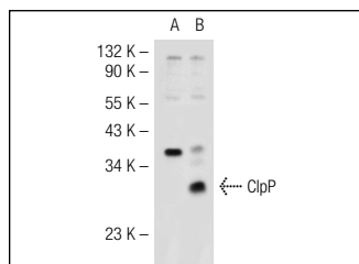
ClpP (C-17): sc-47845. Western blot analysis of ClpP expression in non-transfected: sc-117752 (A) and mouse ClpP transfected: sc-119316 (B) 293T whole cell lysates.
