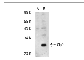
ClpP (C-17): sc-47845. Western blot analysis of ClpP expression in non-transfected: sc-117752 (A) and human ClpP transfected: sc-170292 (B) 293T whole cell lysates.
