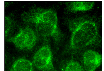
IMP-3 (N-16): sc-47892. Immunofluorescence staining of methanol-fixed HeLa cells showing perinuclear localization.
