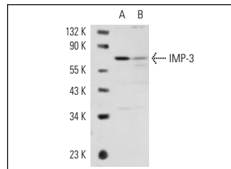
IMP-3 (N-16): sc-47892. Western blot analysis of IMP-3 expression in non-transfected: sc-117752 (A) and human IMP-3 transfected: sc-117068 (B) 293T whole cell lysates.
