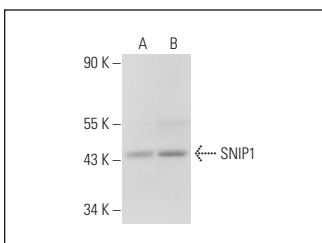
SNIP1 (N-13): sc-47929. Western blot analysis of SNIP1 expression in HeLa whole cell lysate (A) and HeLa nuclear extract (B).
