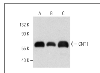
CNT1 (N-17): sc-48460. Western blot analysis of CNT1 expression in human kidney (A), human small intestine (B) and human colon (C) tissue extracts.
