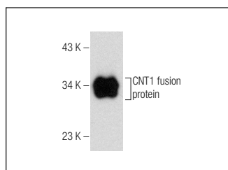
CNT1 (N-17): sc-48460. Western blot analysis of human recombinant CNT1 fusion protein.
