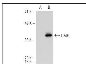
LIME (C-15): sc-48578. Western blot analysis of LIME expression in non-transfected: sc-110760 (A) and human LIME transfected: sc-112792 (B) 293 whole cell lysates.
