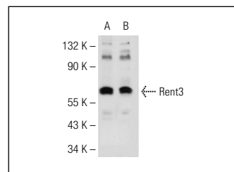
Rent3 (H-190): sc-48800. Western blot analysis of Rent3 expression in SH-SY5Y (A) and MES-SA/Dx5 (B) whole cell lysates.
