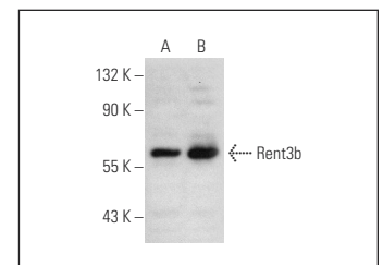
Rent3 (H-190): sc-48800. Western blot analysis of Rent3b expression in non-transfected: sc-117752 (A) and mouse Rent3b transfected: sc-123066 (B) 293T whole cell lysates.
