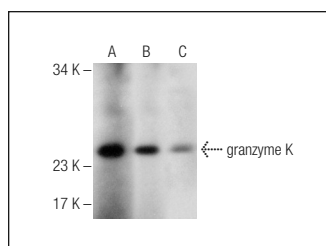
granzyme K (N-12): sc-49023. Western blot analysis of granzyme K expression in RAW 264.7 (A), mouse PBL (B) and M1 (C) whole cell lysates.
