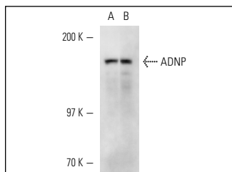
ADNP (E-20): sc-49344. Western blot analysis of ADNP expression in HeLa (A) and SK-N-MC (B) nuclear extracts.
