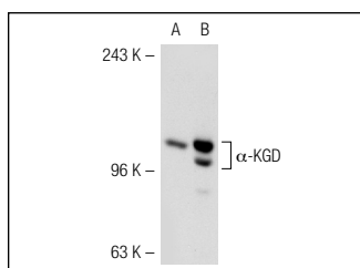
\alpha -KGD (C-20): sc-49589. Western blot analysis of \alpha -KGD expression in non-transfected: sc-117752 (A) and mouse \alpha -KGD transfected: sc-124905 (B) 293T whole cell lysates.
