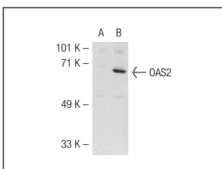
OAS2 (M-18): sc-49858. Western blot analysis of OAS2 expression in non-transfected: sc-117752 (A) and human OAS2 transfected: sc-116044 (B) 293T whole cell lysates.
