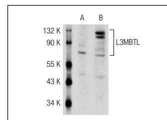
L3MBTL (C-20): sc-50038. Western blot analysis of L3MBTL expression in non-transfected: sc-117752 (A) and human L3MBTL transfected: sc-115550 (B) 293T whole cell lysates.
