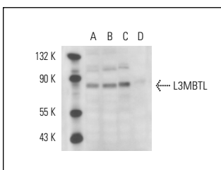
L3MBTL (C-20): sc-50038. Western blot analysis of L3MBTL expression in HEL 92.1.7 (A), CCRF-CEM (B) and SK-N-MC (C) nuclear extracts and U-87 MG whole cell lysate (D).
