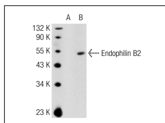
Endophilin B2 (T-14): sc-50572. Western blot analysis of Endophilin B2 expression in non-transfected: sc-117752 (A) and human Endophilin B2 transfected: sc-177187 (B) 293T whole cell lysates.
