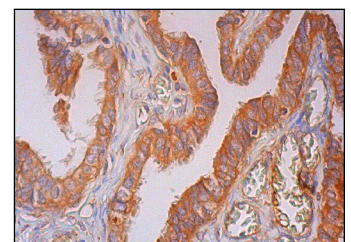
NALP7 (L-19): sc-50641. Immunoperoxidase staining of formalin fixed, paraffin-embedded human fallopian tube tissue showing cytoplasmic staining of glandular cells.
