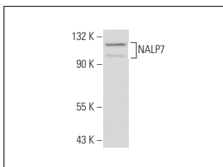
NALP7 (L-19): sc-50641. Western blot analysis of NALP7 expression in Jurkat whole cell lysate.
