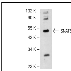
SNAT5 (N-15): sc-50681. Western blot analysis of SNAT5 expression in Sol8 whole cell lysate.
