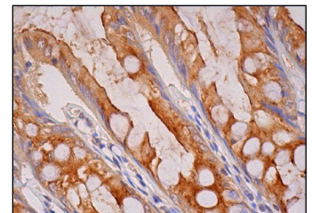
SNAT5 (N-15): sc-50681. Immunoperoxidase staining of formalin fixed, paraffin-embedded human rectum tissue showing cytoplasmic and membrane staining of glandular cells.
