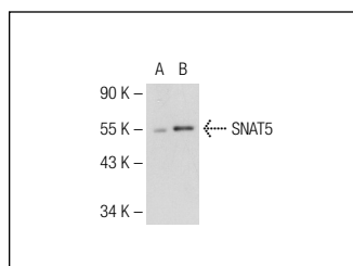
SNAT5 (Q-15): sc-50682. Western blot analysis of SNAT5 expression in non-transfected: sc-117752 (A) and human SNAT5 transfected: sc-173683 (B) 293T whole cell lysates.
