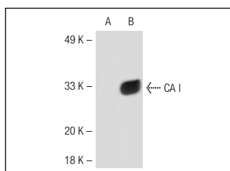
CA I (N-16): sc-50898. Western blot analysis of CA I expression in non-transfected: sc-117752 (A) and human CA I transfected: sc-114146 (B) 293T whole cell lysates.
