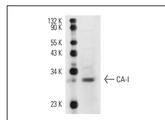
CA I (N-16): sc-50898. Western blot analysis of CA I expression in K-562 whole cell lysate.
