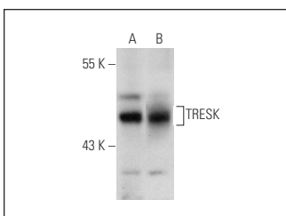
TRESK (P-19): sc-51238. Western blot analysis of TRESK expression in Hep G2 (A) and HeLa (B) whole cell lysates.
