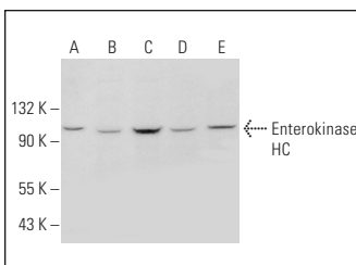
Enterokinase HC (V-20): sc-51281. Western blot analysis of Enterokinase HC expression in HeLa (A), Jurkat (B), K-562 (C), Hep G2 (D) and NIH/3T3 (E) whole cell lysates.
