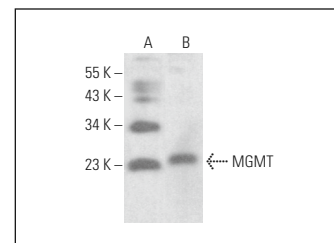
MGMT (G-10): sc-514277. Western blot analysis of MGMT expression in HeLa (A) and MDA-MB-435S (B) whole cell lysates.
